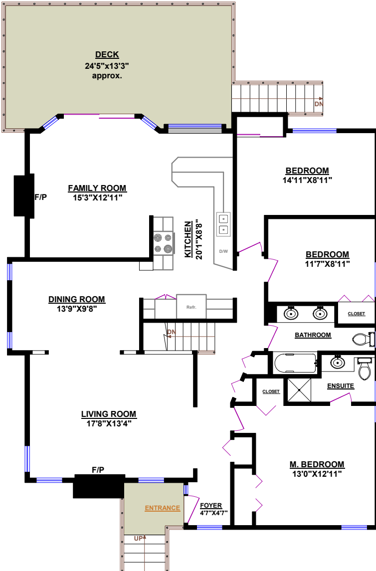
MAIN FLOOR
