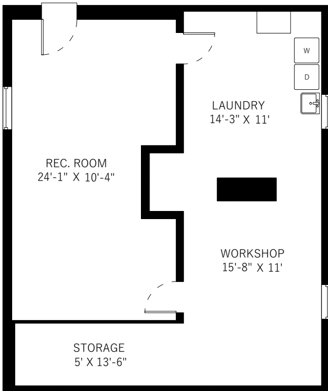
Unfinished Lower Floor: 813 Sq.Ft. Ceiling Height: 6'-5"
