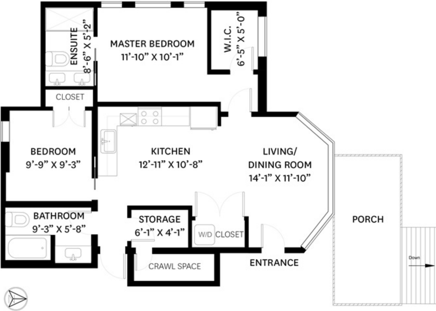
MAIN FLOOR PLAN Ceiling Height: 10'-5"
