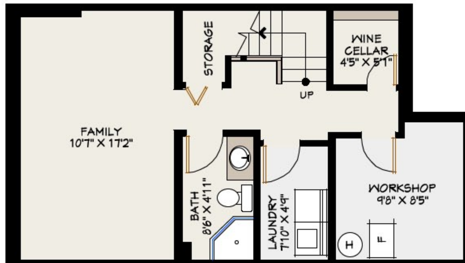
LOWER LEVEL
