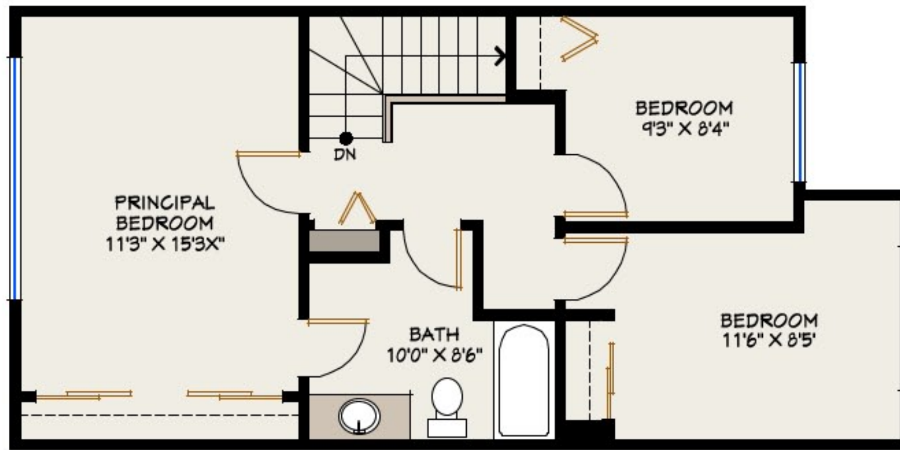
UPPER LEVEL
