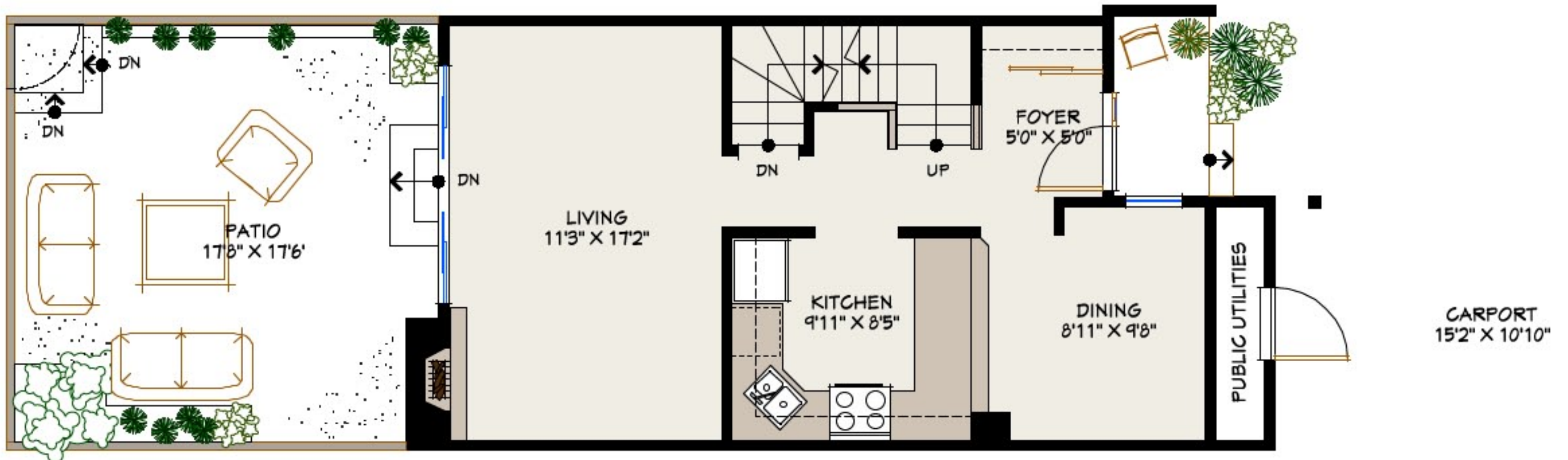
MAIN LEVEL
