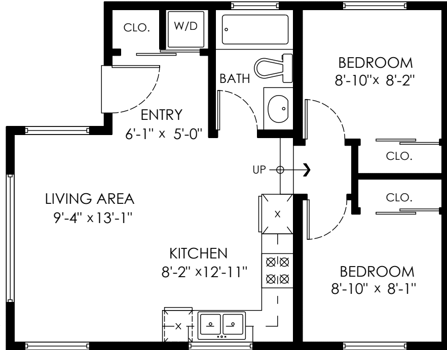
Laneway House Floor Plan Floor Area: 566 sq.ft.
