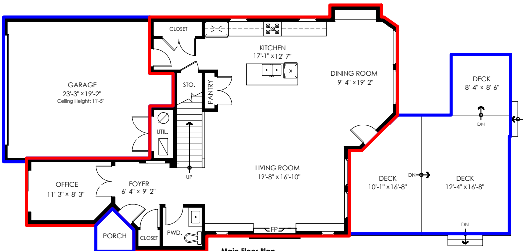
Main Floor Plan Floor Area: 1154 sq.ft. Ceiling Height: 10'-0"
