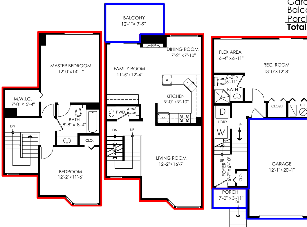
Upper Floor Plan Floor Area: 590 sq.ft. Ceiling Height: 7'-11"
