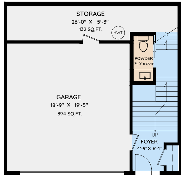
LOWER FLOOR 187 SQ.FT. CH: 12'-0"
