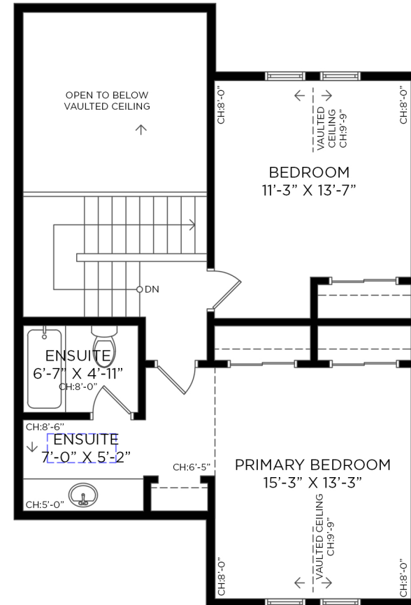
UPPER FLOOR - 582 SQ.FT. CEILING HEIGHT: 5'-0" TO 9'-9"
