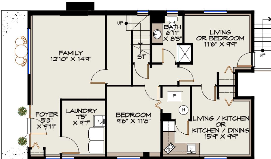
LOWER LEVEL - LARGE ONE OR TWO BEDROOM SUITE
