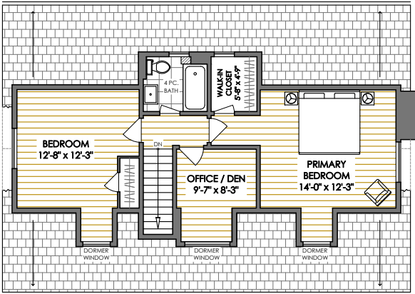
UPPER FLOOR 630 SQ.FT 5'-0" TO 7'-8" CEILING HEIGHT
