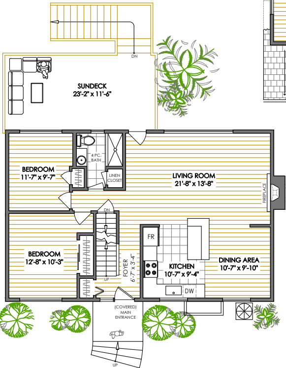
MAIN FLOOR 1040 SQ.FT 8'-0" CEILING HEIGHT
