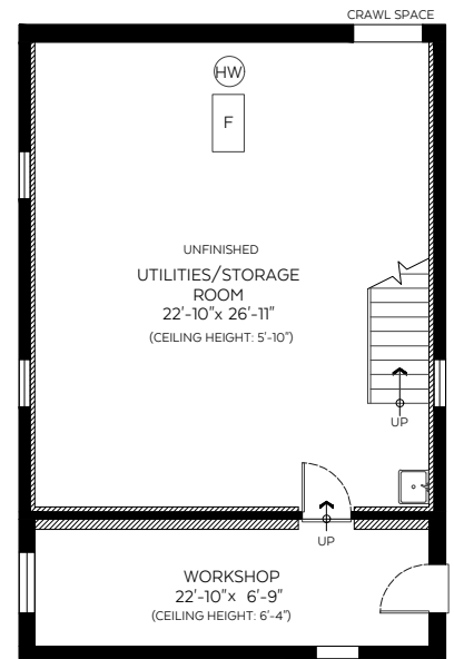
Lower Floor Plan Floor Area: 907 sq.ft.
