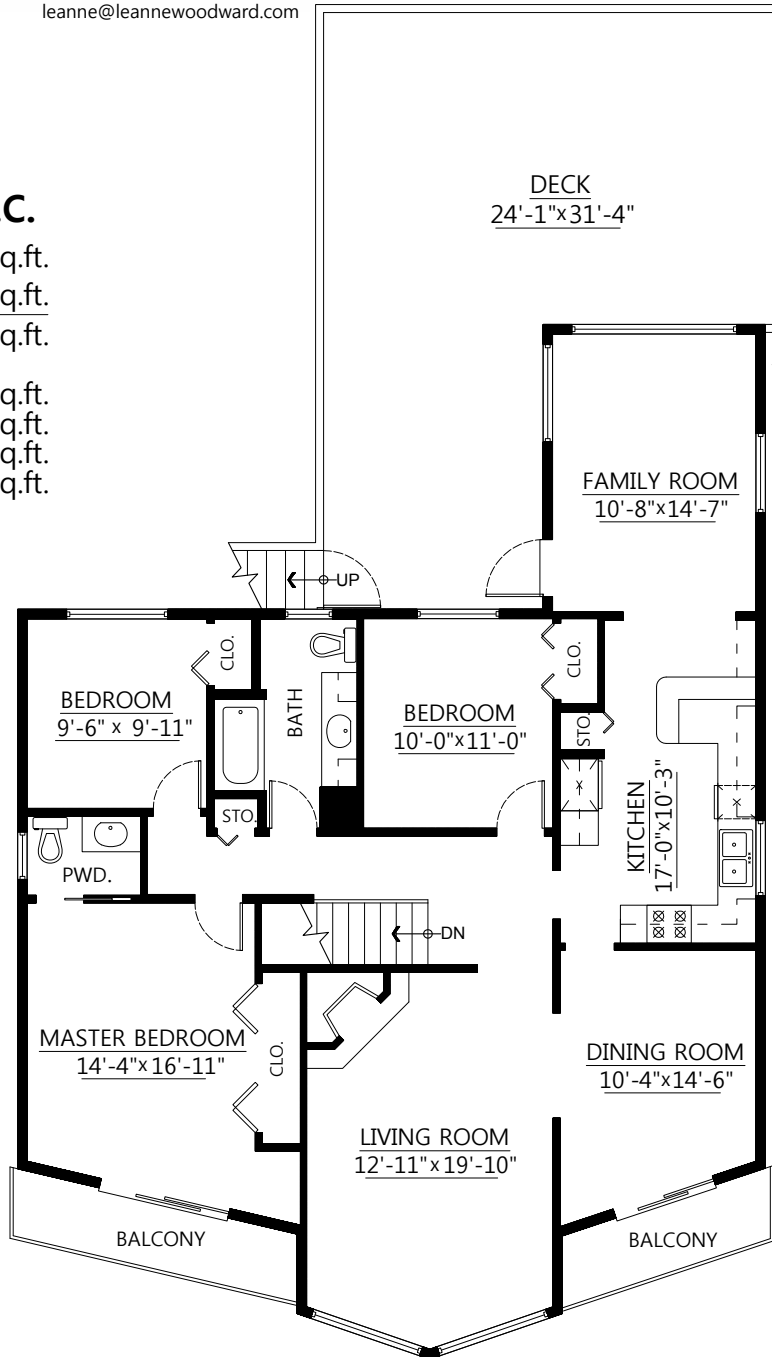
Lower Floor Plan Floor Area: 1,501 sq.ft.
