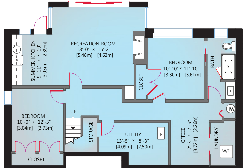
LOWER FLOOR PLAN Floor Area: 1313 sq.ft. Floor Area: 121.98 sq.m.
