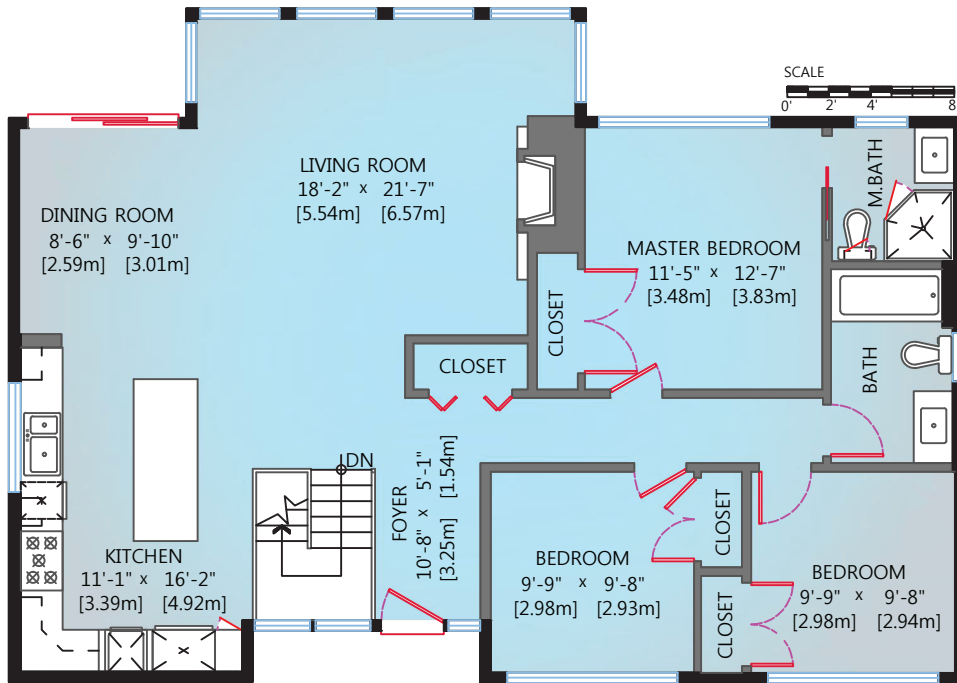
MAIN FLOOR PLAN Floor Area: 1313 sq.ft. Floor Area: 121.98 sq.m.
