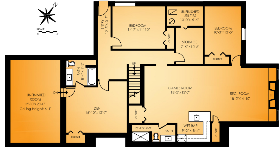
Lower Floor Plan Finished Area: 1941 sq.ft. Ceiling Height: 7'-11" Unfinished Area: 460 sq.ft.
