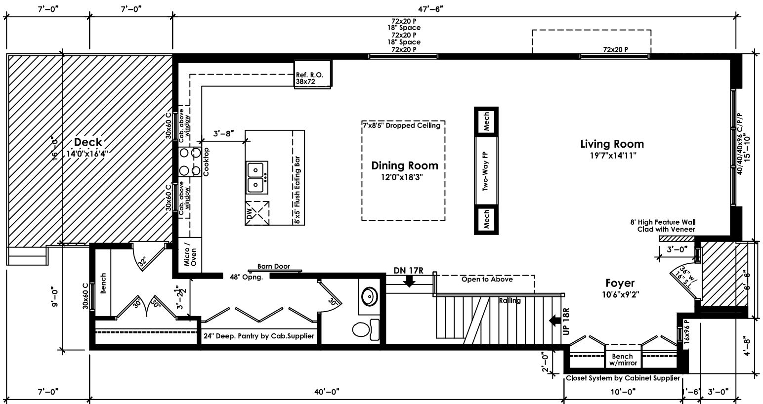
Main Floor Plan - 1 1239 sf (10'-1" Ceiling)
