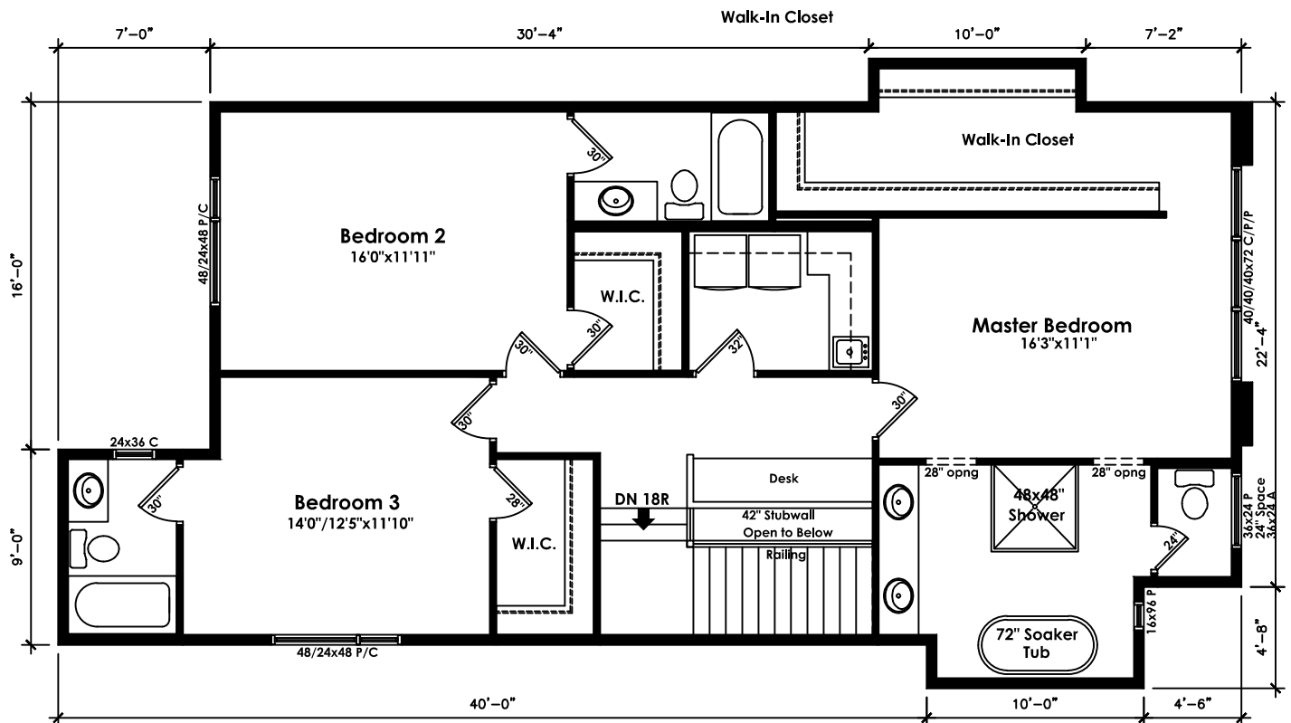
Second Floor Plan - 1 1205 sf (9'-1" Ceiling)
