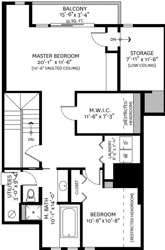
UPPER FLOOR PLAN Ceiling Height: 8'-0"
