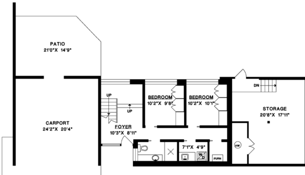
LOWER FLOOR
