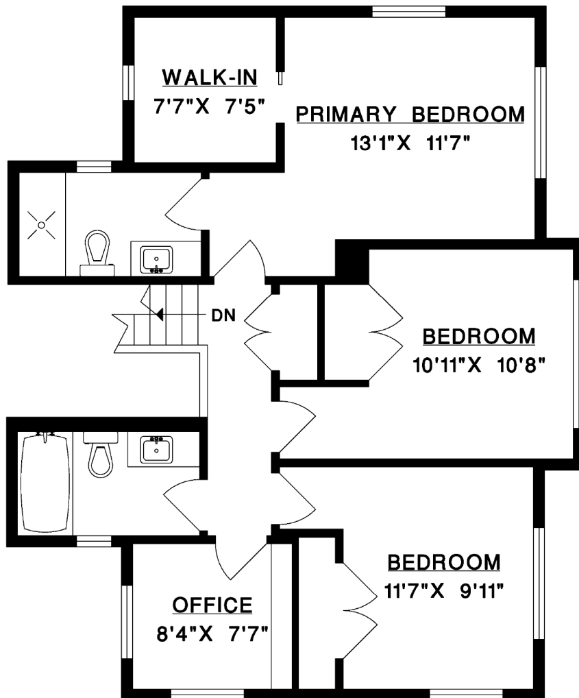
UPPER FLOOR
