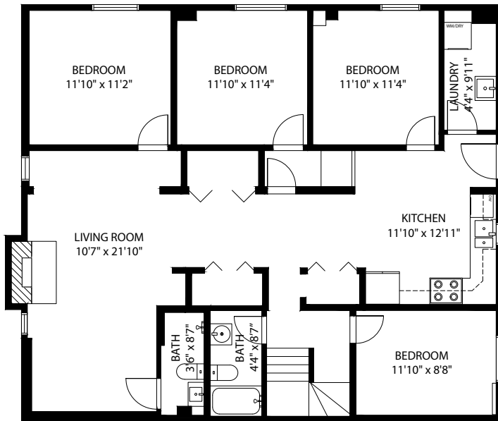
Lower Level: 1,366 sq.ft. Ceiling Height: 7'8"
