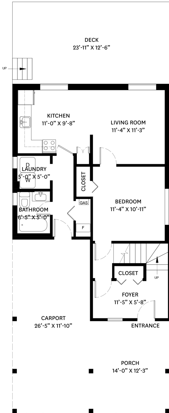
LOWER FLOOR PLAN Ceiling Height: 7'-9"
