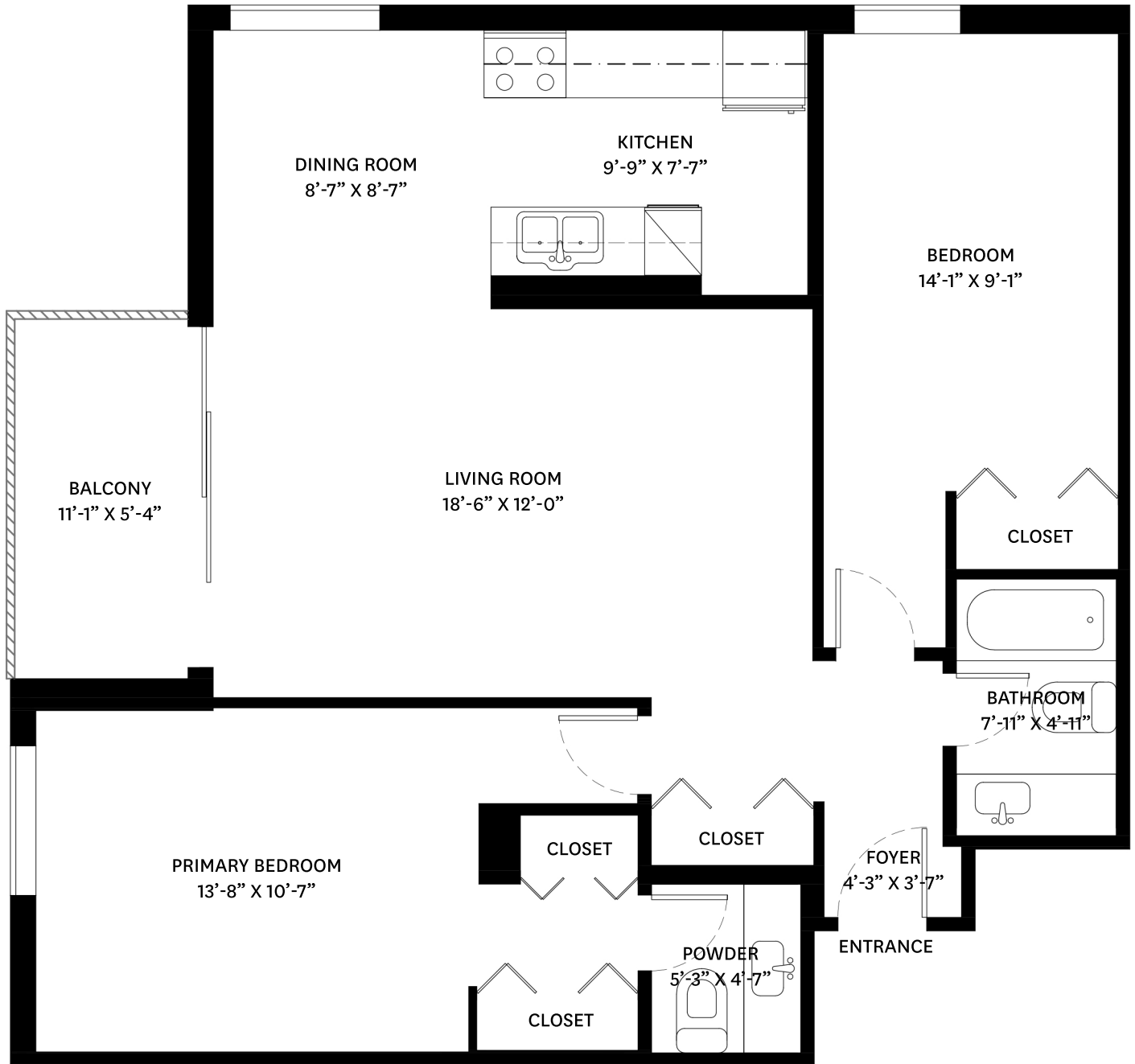
MAIN FLOOR PLAN Ceiling Height: 7'-11"
