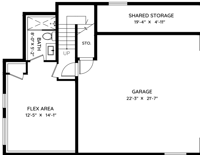
LOWER FLOOR 412.2 SQ.FT.
