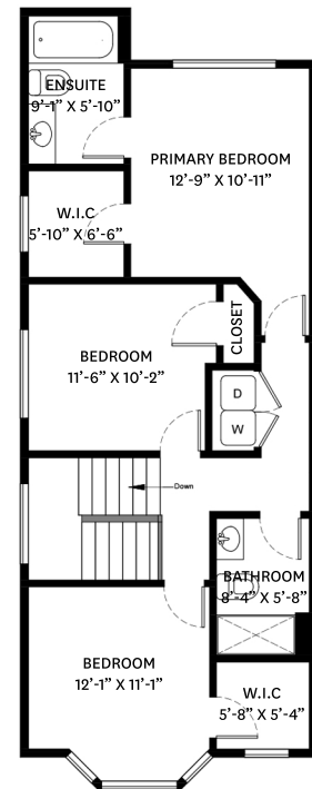
UPPER FLOOR PLAN Ceiling Height: 8'-0"
