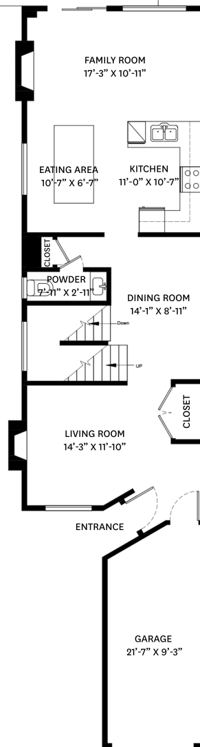
MAIN FLOOR PLAN Ceiling Height: 8'-11"
