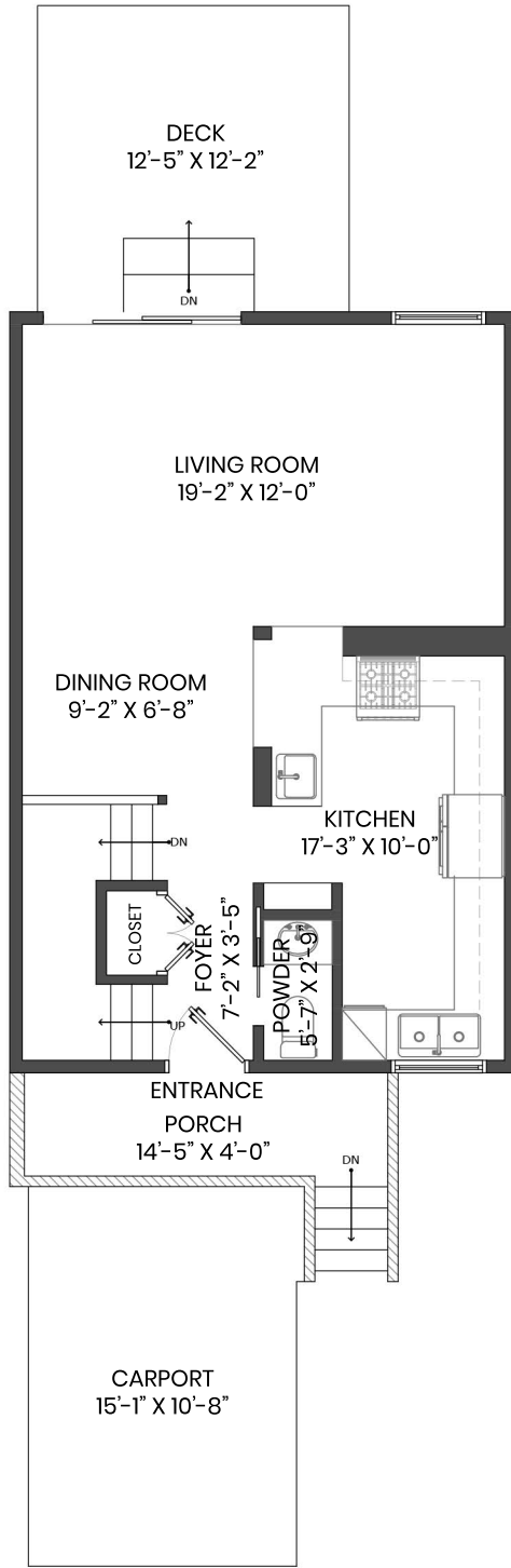
MAIN FLOOR PLAN Ceiling Height: 8'-0"
