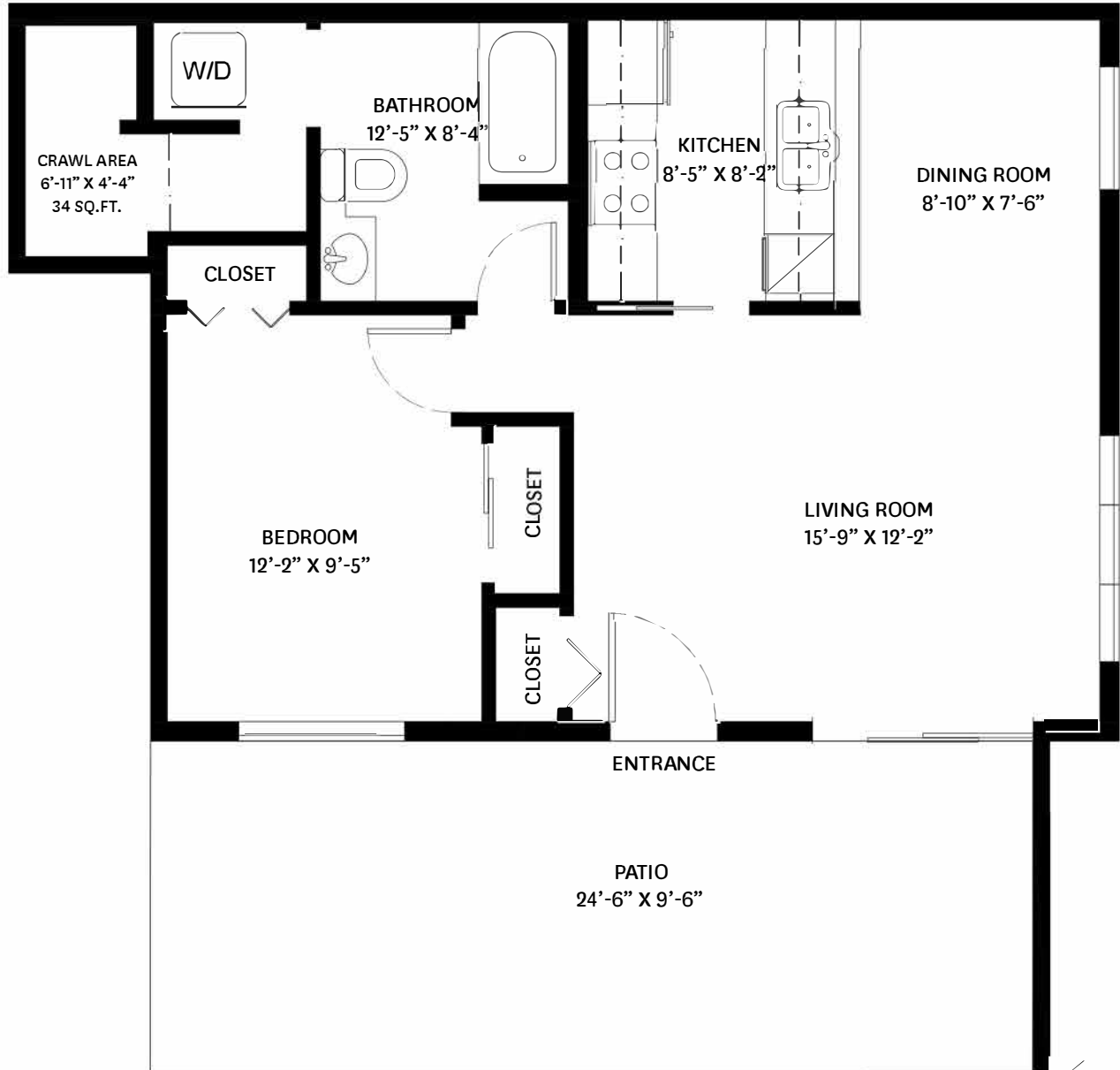
MAIN FLOOR PLAN Ceiling Height: 7'-11"
