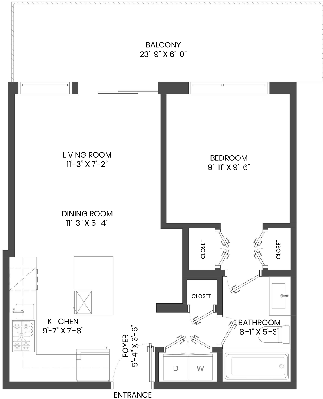
MAIN FLOOR PLAN Ceiling Height: 9'-0"
