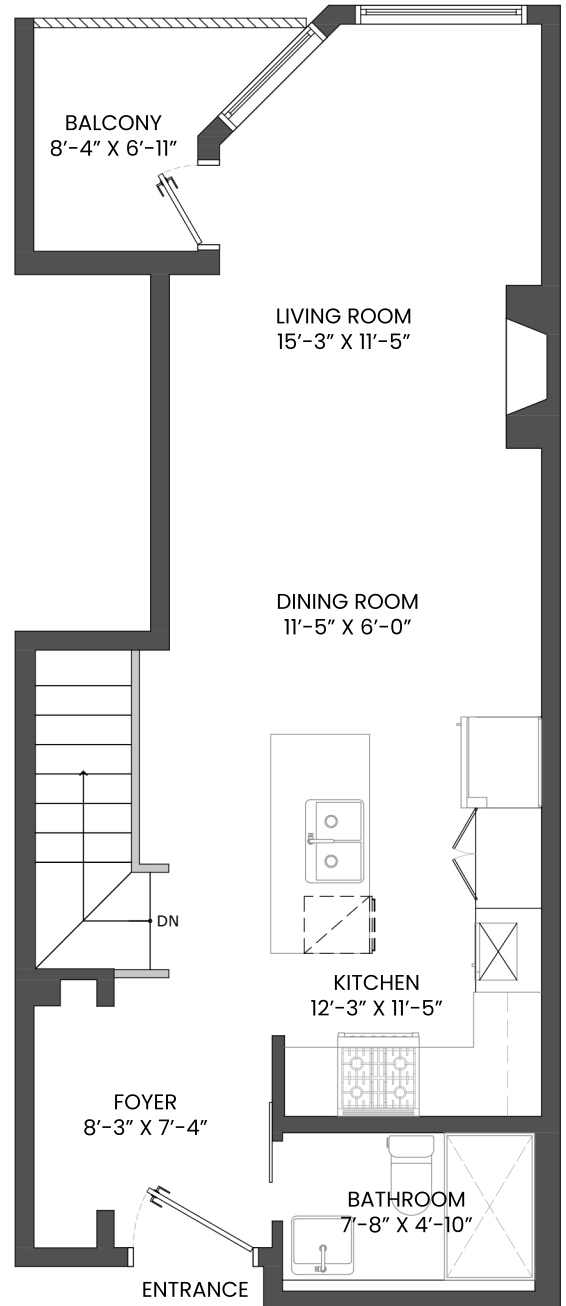
MAIN FLOOR PLAN Ceiling Height: 8'-0"
