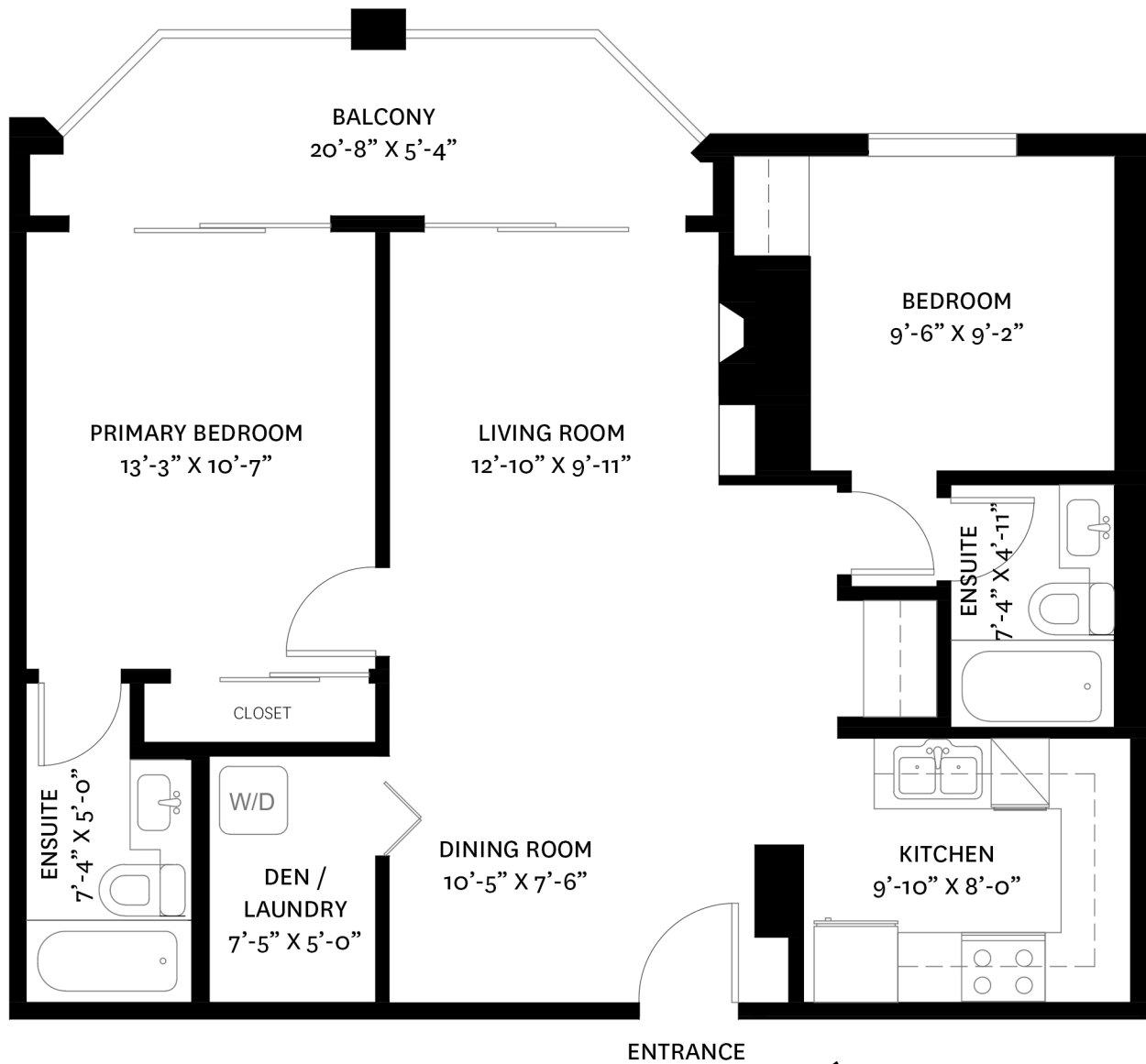
MAIN FLOOR PLAN Ceiling Height: 8'-0"
