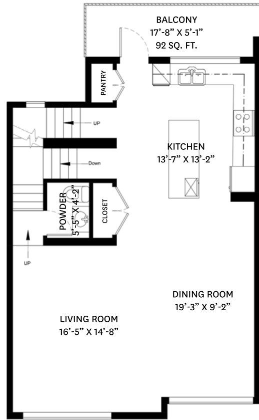
MAIN FLOOR PLAN Ceiling Height: 8'-11"
