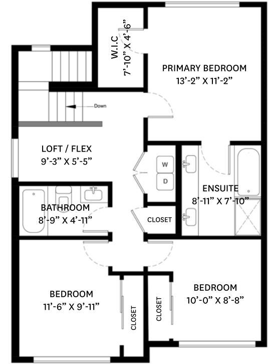
UPPER FLOOR PLAN Ceiling Height: 9'-0"
