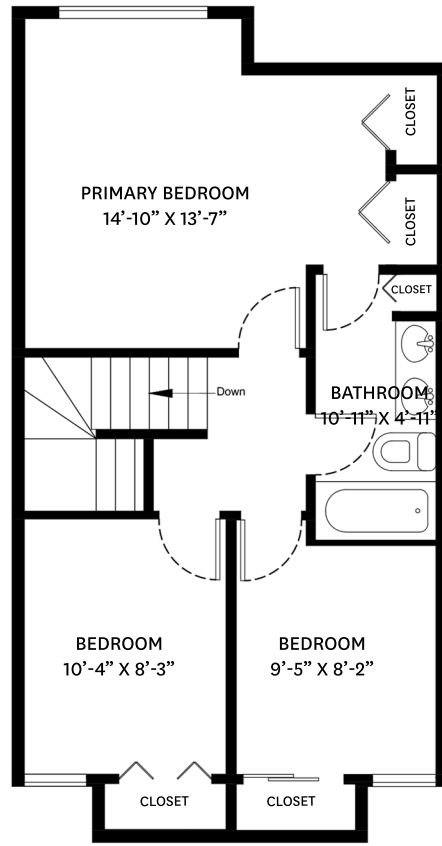
UPPER FLOOR PLAN Ceiling Height: 8'-0"
