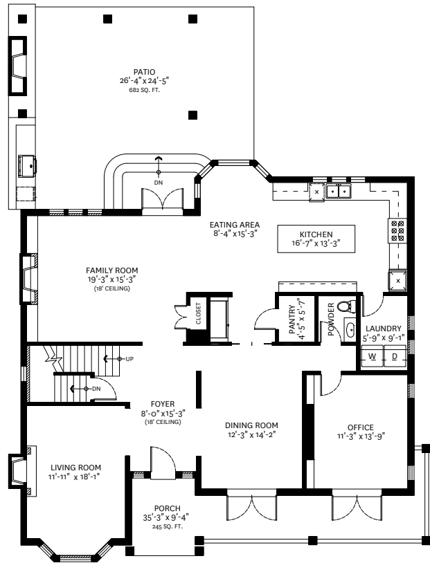
MAIN FLOOR PLAN Ceiling Height: 8'-10"
