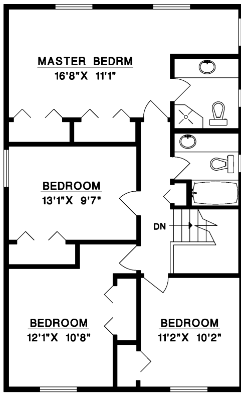
UPPER FLOOR
