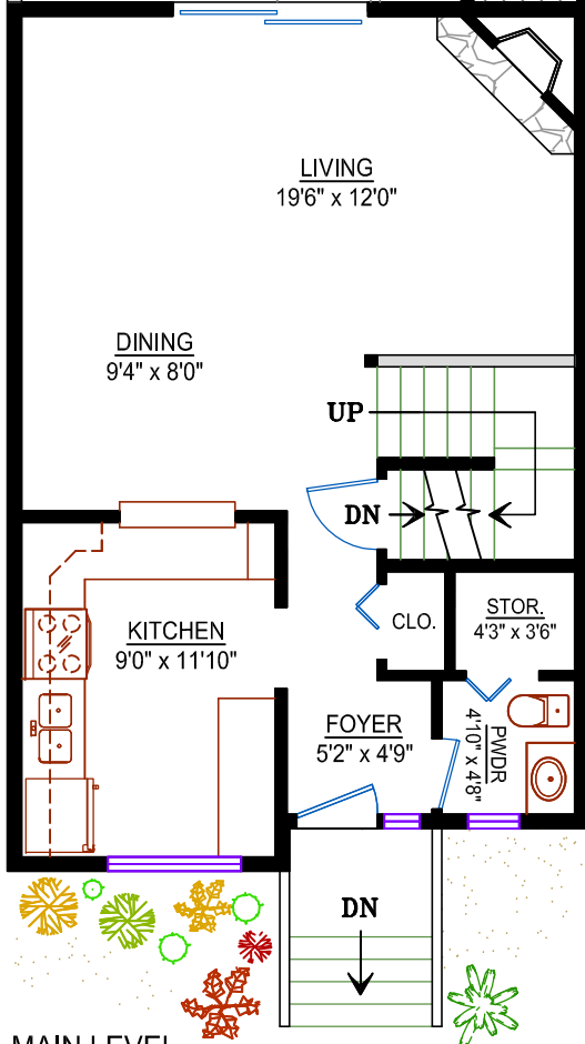
MAIN LEVEL Area: 602 sq. ft.
