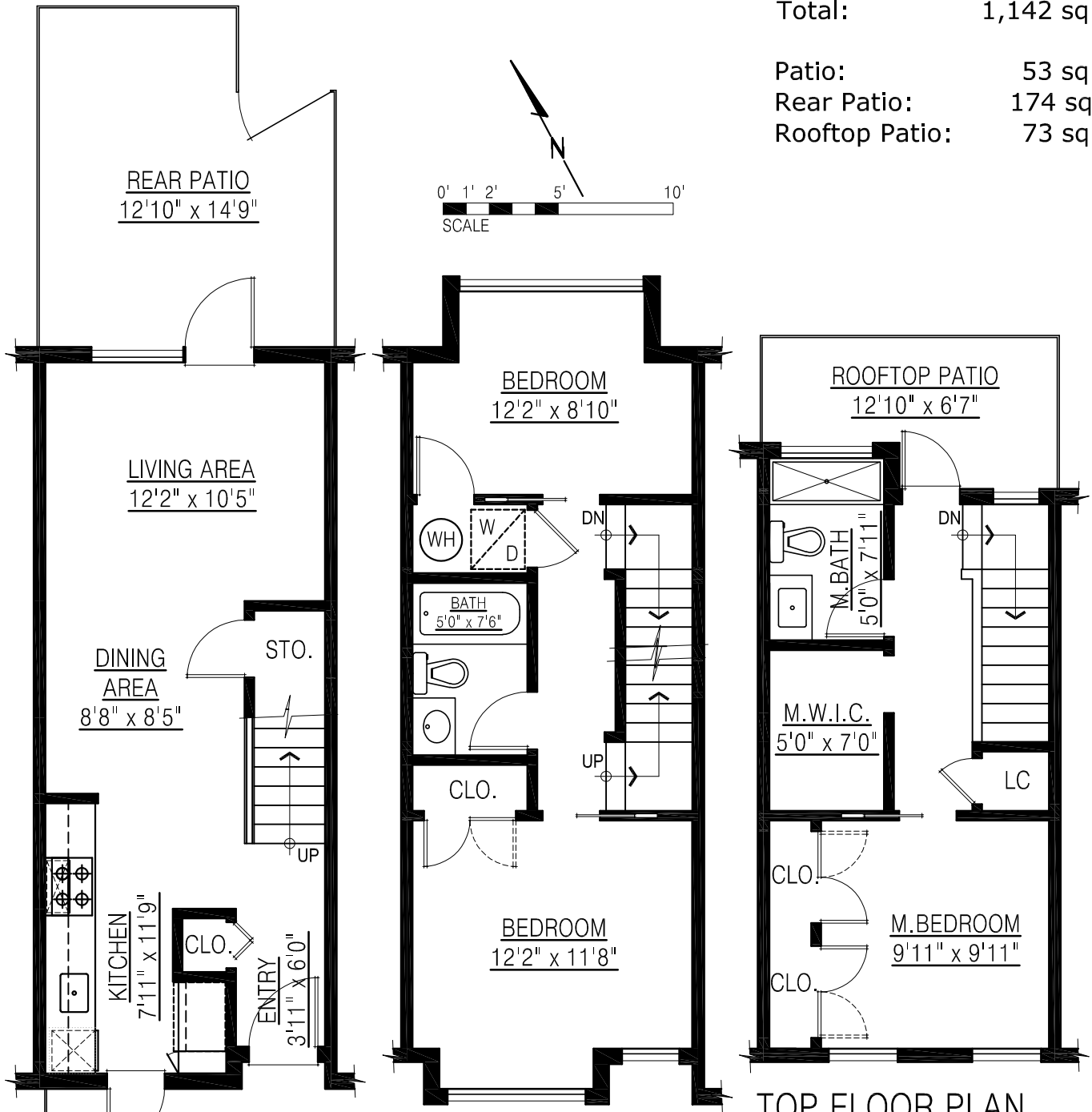
UPPER FLOOR PLAN FLOOR AREA: 426 sq.ft.
