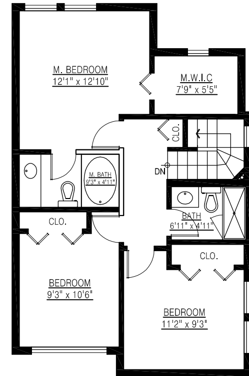
UPPER FLOOR PLAN FLOOR AREA: 673 sq. ft.
