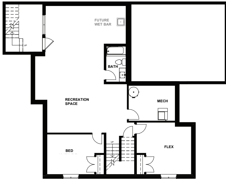
Standard Finished Basement 1,343 SQ.FT.
