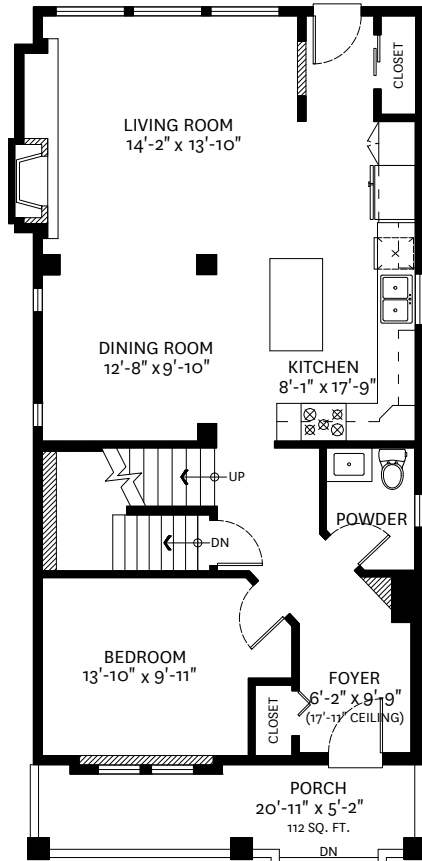
MAIN FLOOR PLAN Ceiling Height: 8'-11"
