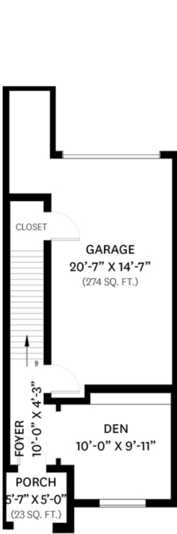
LOWER FLOOR PLAN Ceiling Height: 8'-0"
