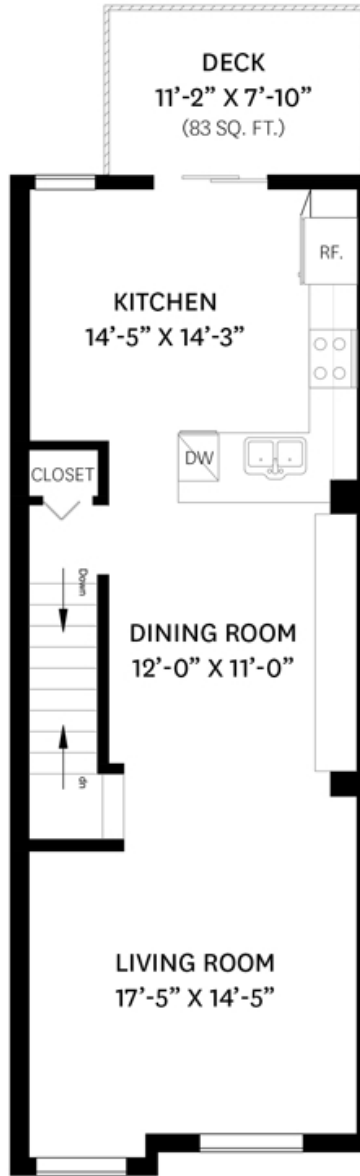
MAIN FLOOR PLAN Ceiling Height: 9'-0"
