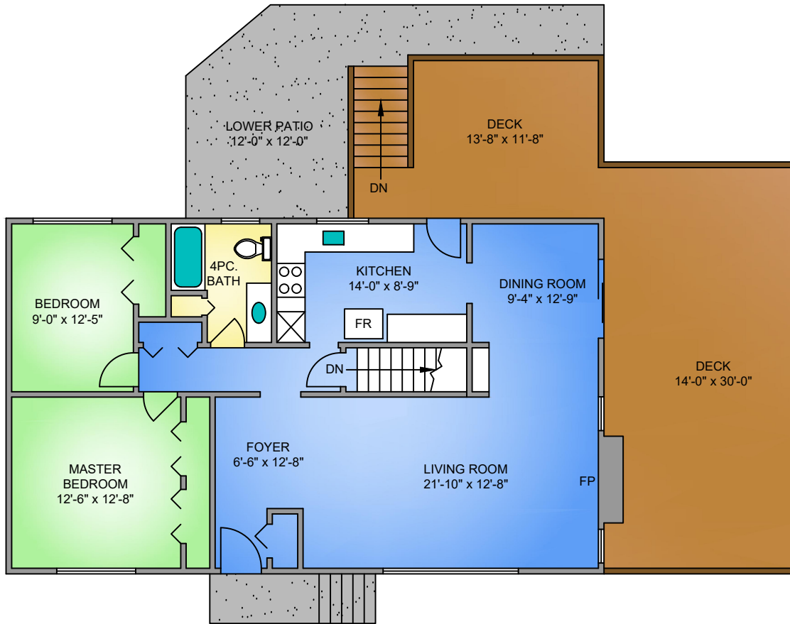
MAIN FLOOR 1163 SQ. FT. 8FT. CEILING
