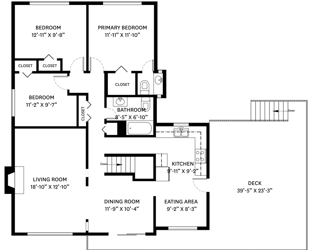
MAIN FLOOR PLAN Ceiling Height: 8'-0"
