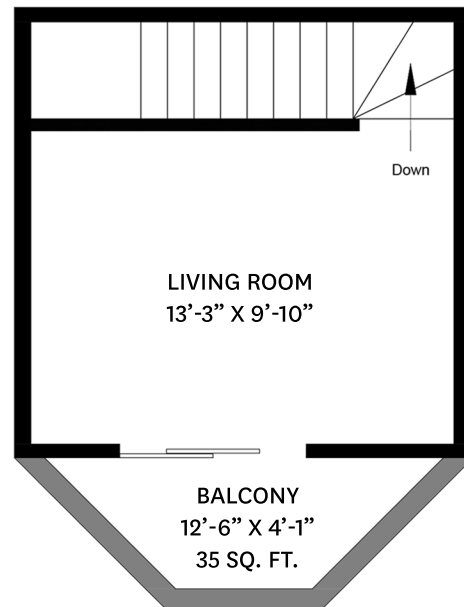
UPPER FLOOR PLAN Ceiling Height: 7'-10"
