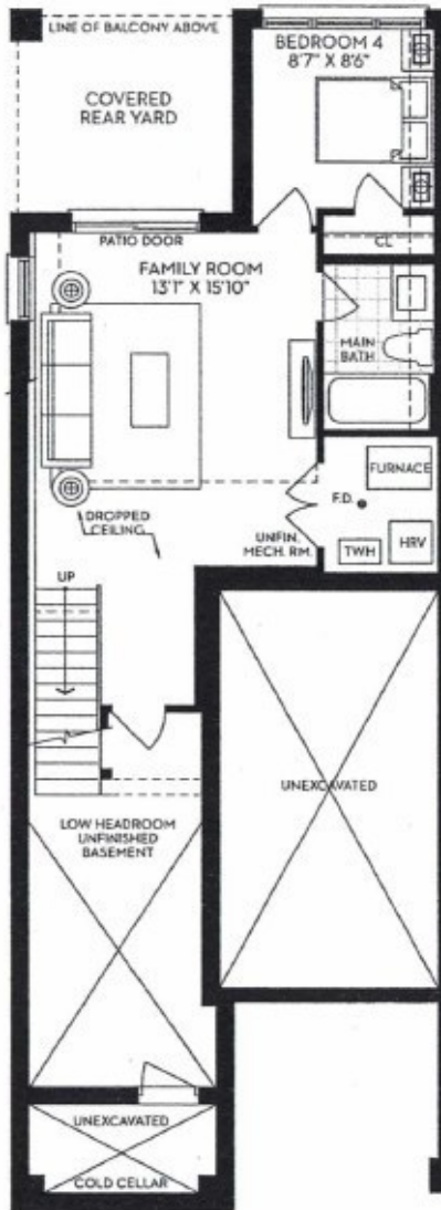
BASEMENT PLAN ELEVATION 'SIC'
