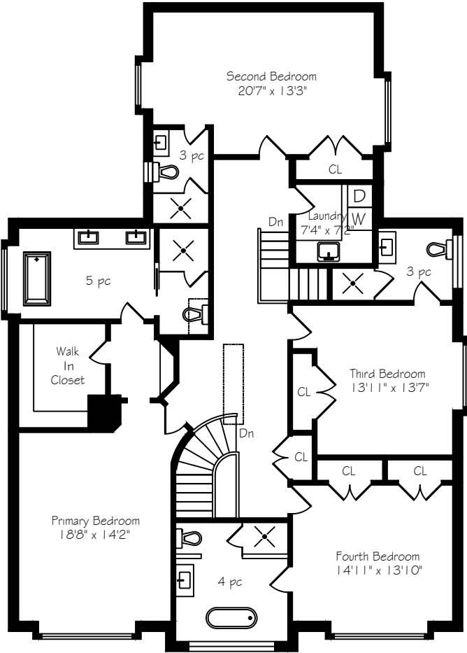
Second Floor 2118 Square Feet
