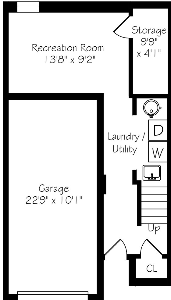
Lower Level 370 Square Feet + 238 Garage
