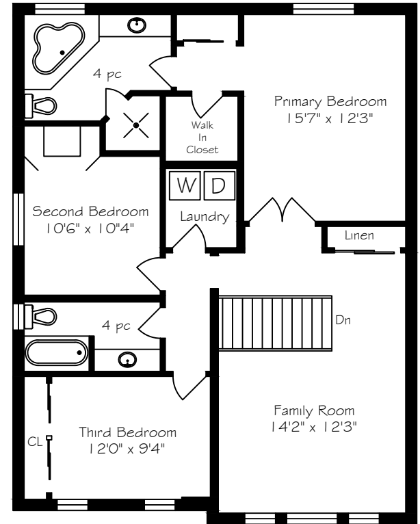
Second Floor 1184 Square Feet
