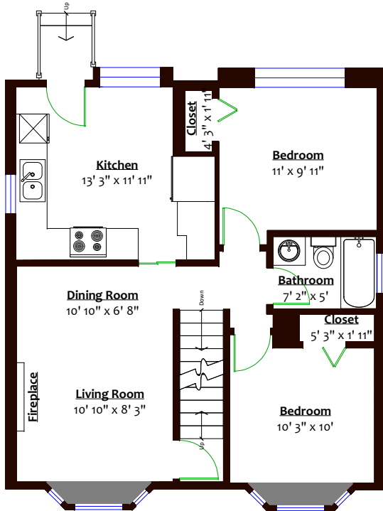
MAIN LEVEL Floor Area: 775 Sq. Ft.
