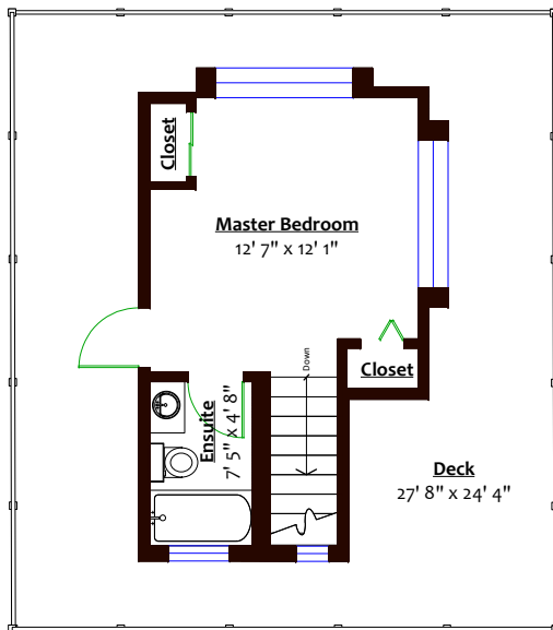
UPPER LEVEL Floor Area: 265 Sq. Ft.
