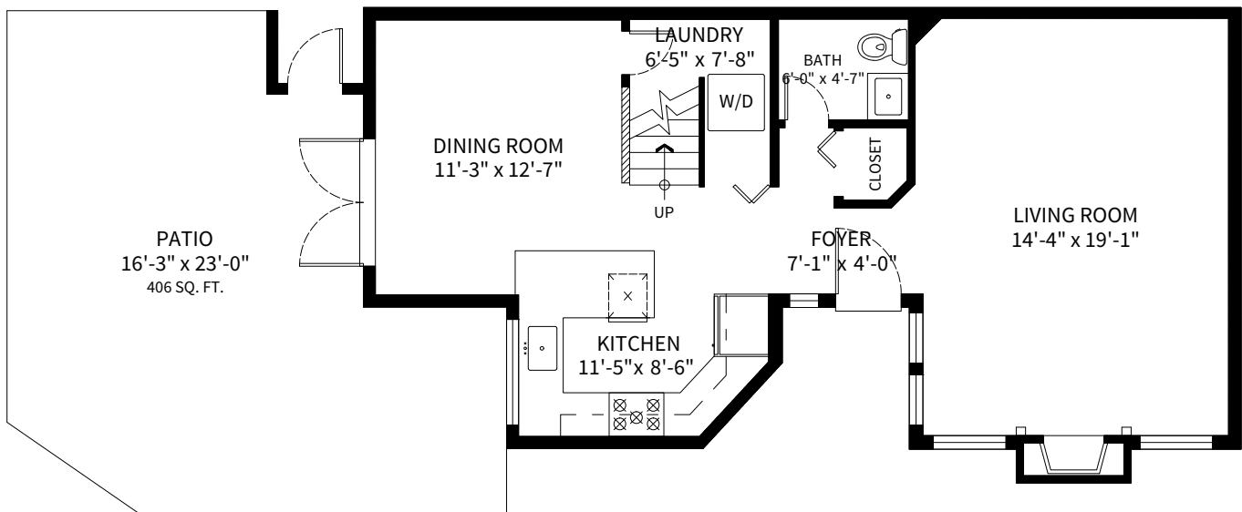
MAIN FLOOR PLAN Ceiling Height: 8'-0"
