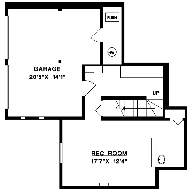
LOWER FLOOR
