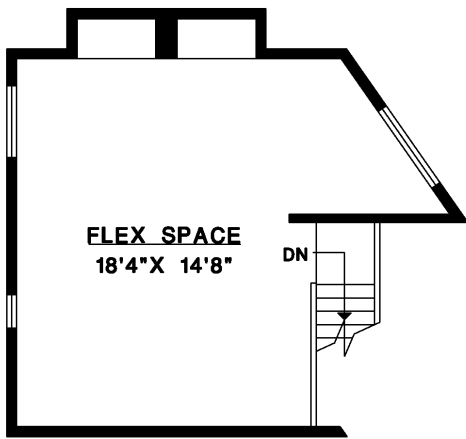
UPPER FLOOR
